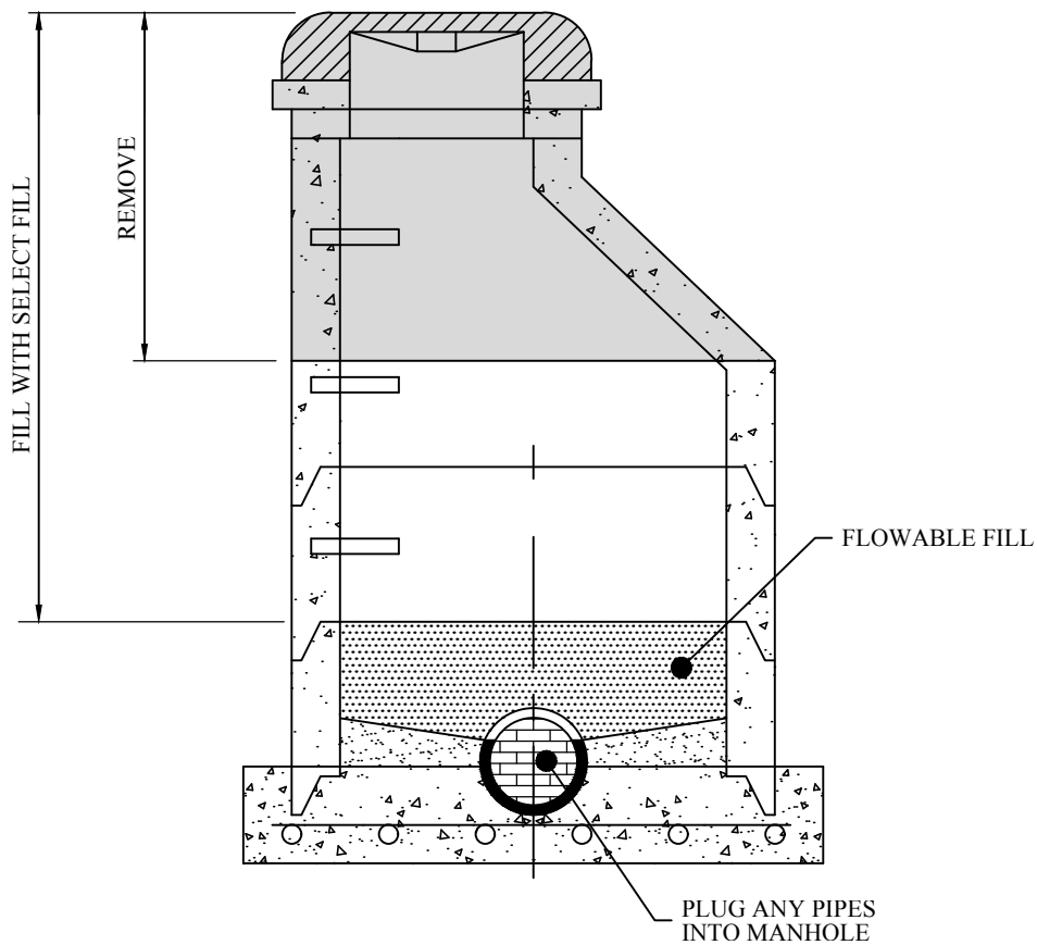
PROFILE VIEW
