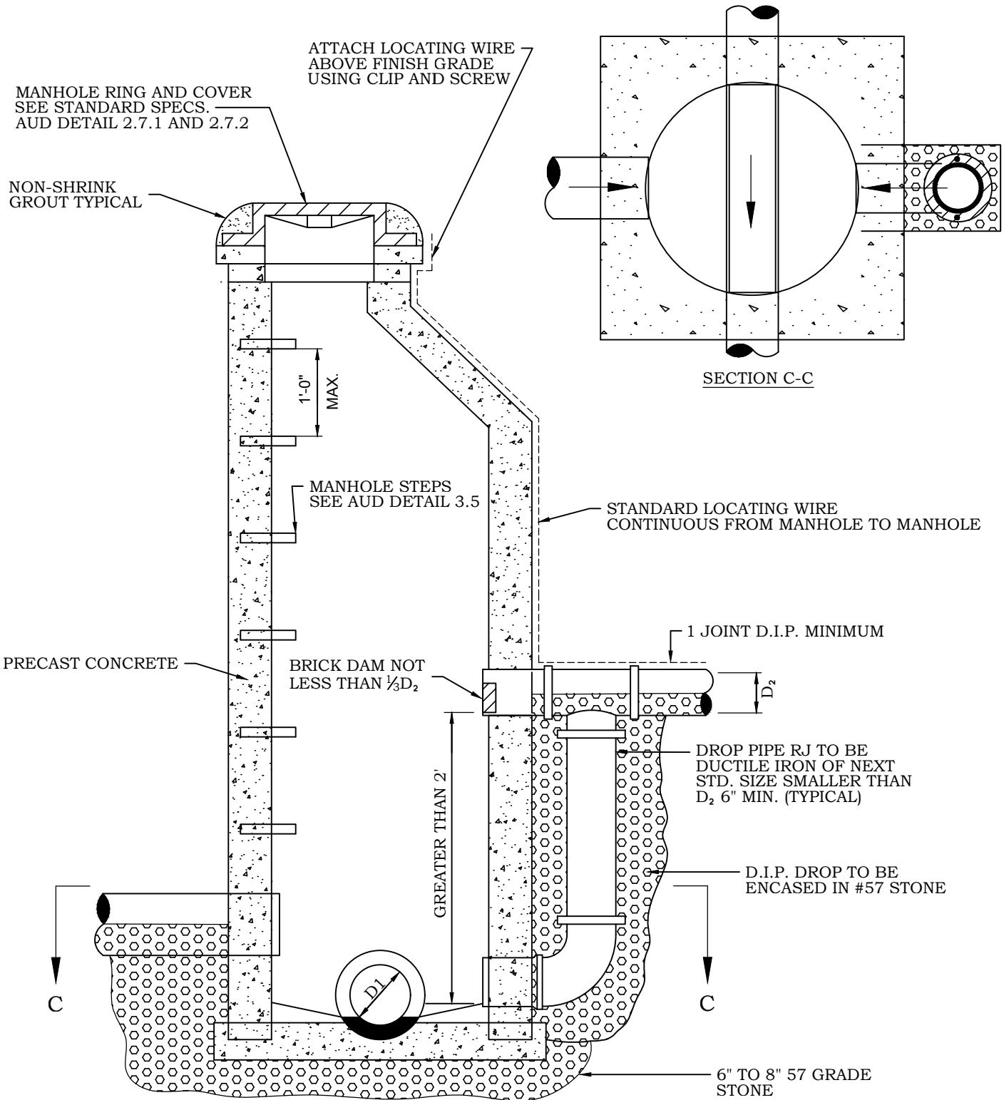
TYPICAL SECTION
