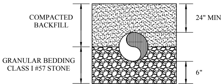
STONE BEDDING
