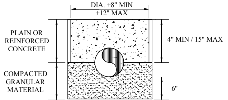
CONCRETE ARCH
