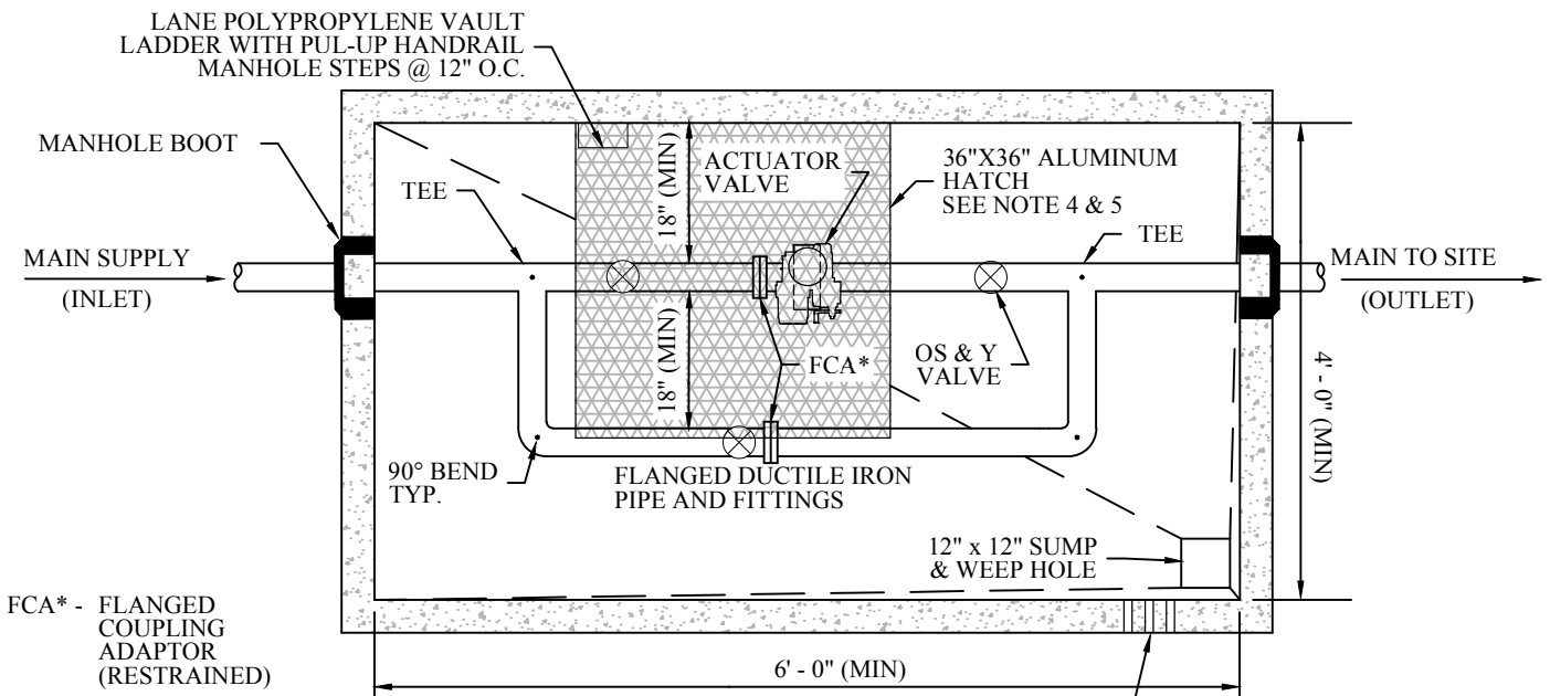
PLAN VIEW
