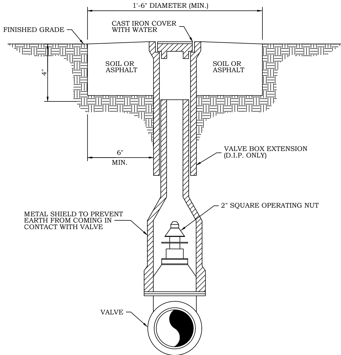
PROFILE VIEW
