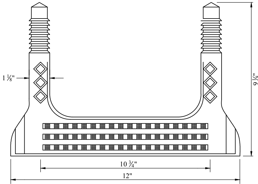
PLAN VIEW
