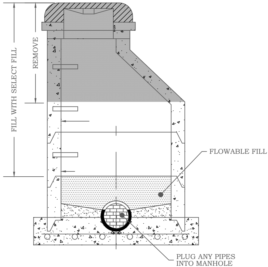
PROFILE VIEW
