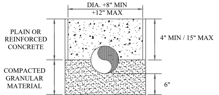
CONCRETE ARCH
