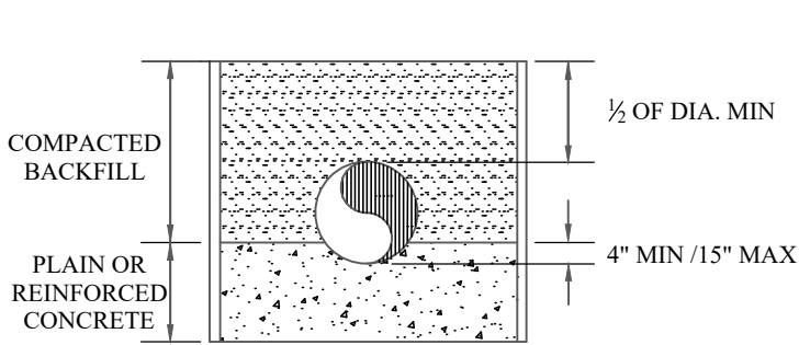
CONCRETE CRADLE
