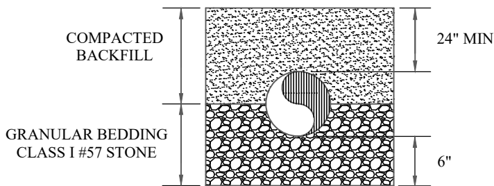
STONE BEDDING
