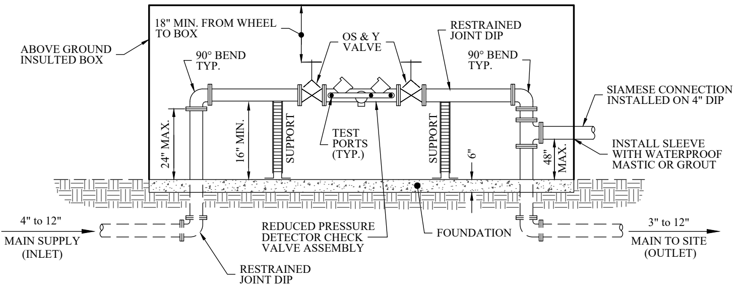
PROFILE VIEW
