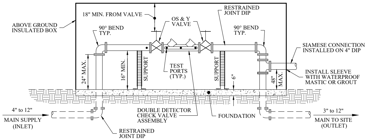
PROFILE VIEW
