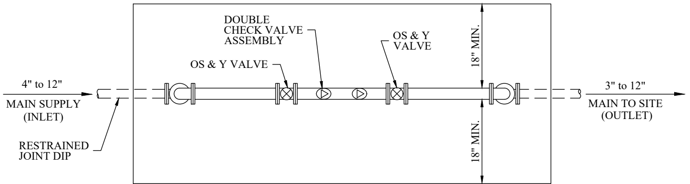
PLAN VIEW
