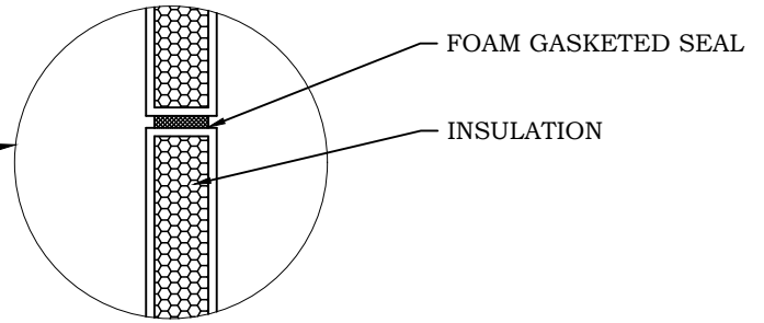
SIDE VIEW OF LIP SEAL
