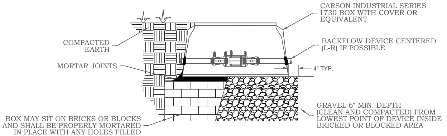
INSTALLATION #1 PROFILE VIEW
