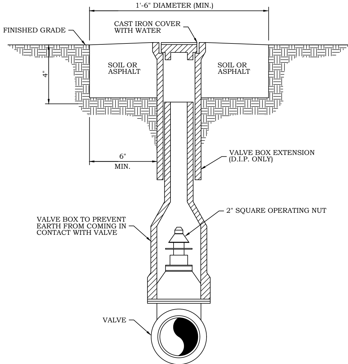
PROFILE VIEW
