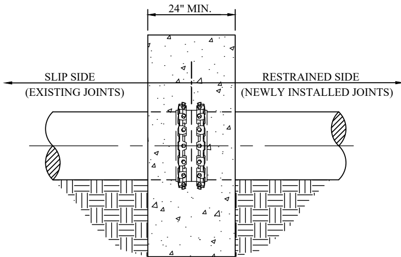
PROFILE VIEW
