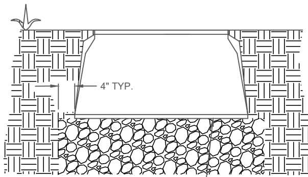
PROFILE VIEW
