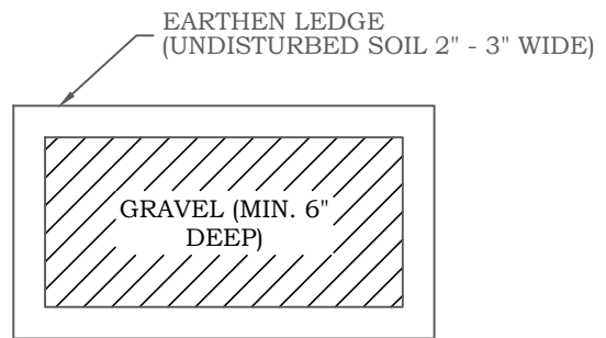
LEDGE DETAIL
