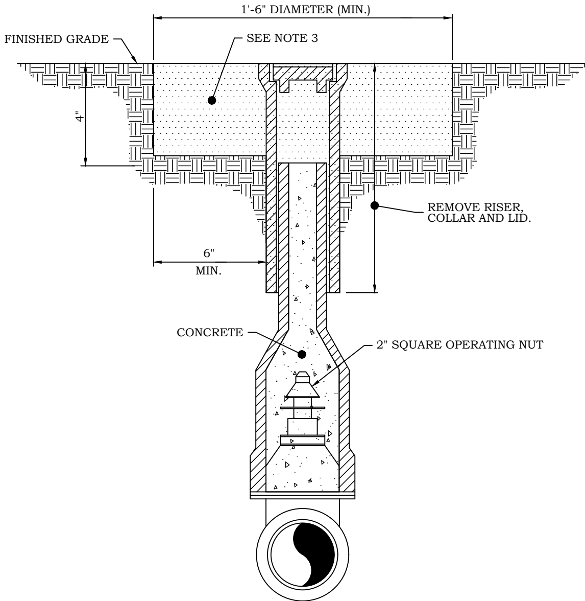
PROFILE VIEW
