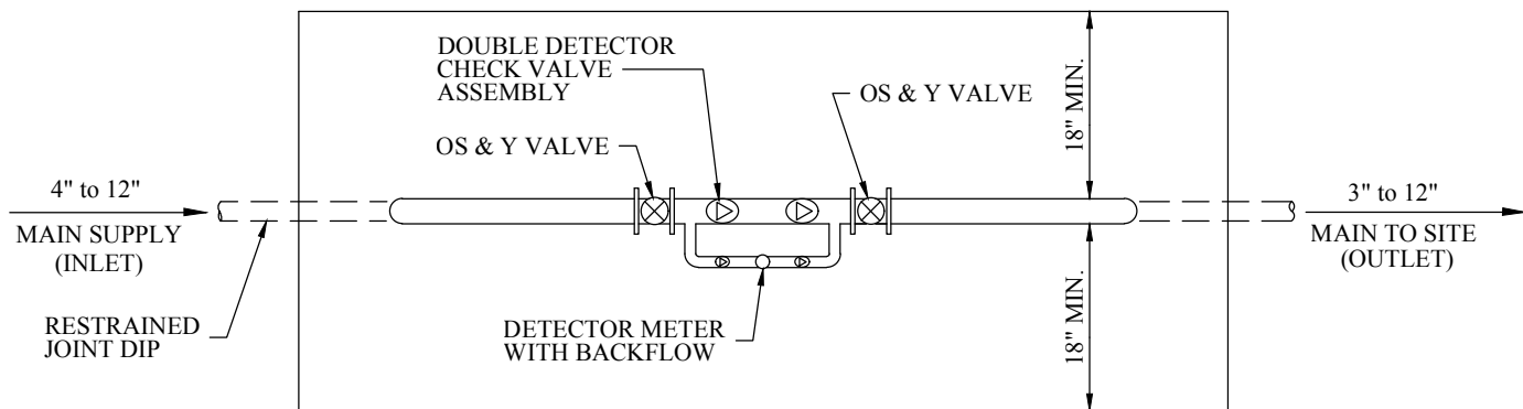
PLAN VIEW
