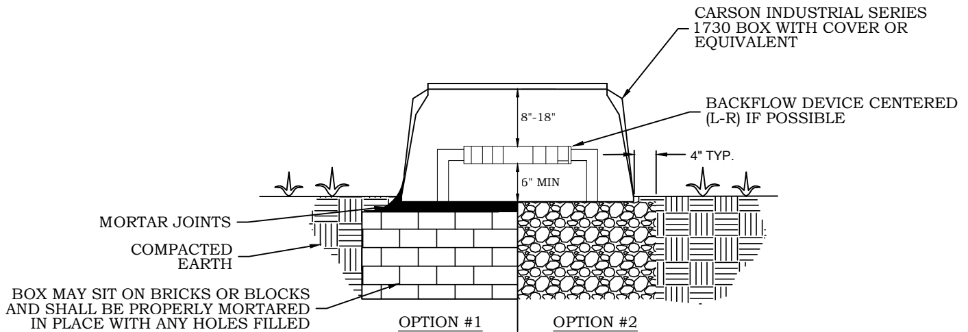
PROFILE VIEW
